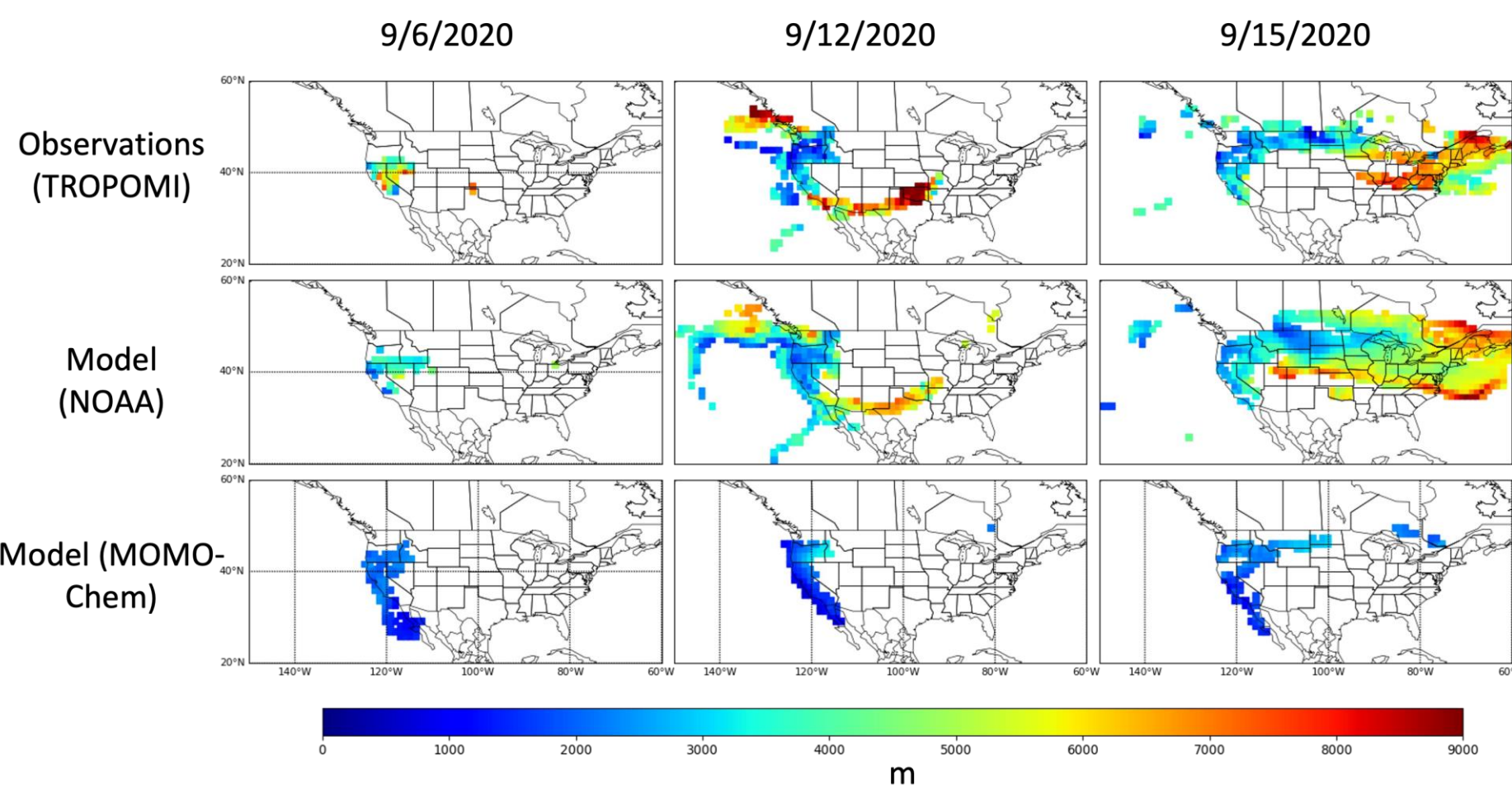
Figure 2: Spatial maps of aerosol scattering heights for TROPOMI retrieval (top), NOAA's RAP-Chem simulation (middle), and MOMO-Chem simulation (bottom).
