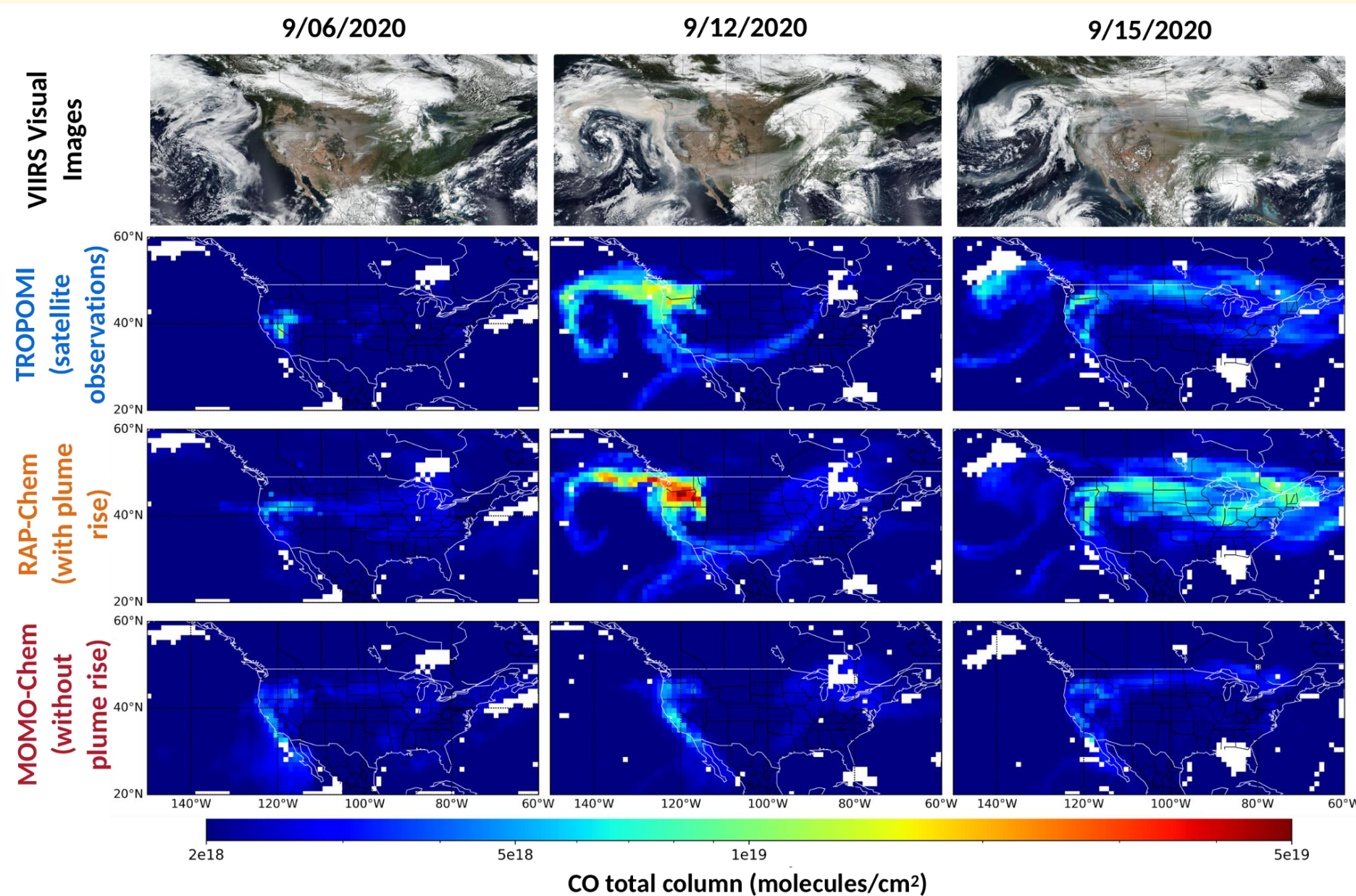
Figure 1: Spatial maps of VIIRS Visual images (1 st row) total CO column for TROPOMI retrieval (2 nd row), NOAA's RAP-Chem simulation with TROPOMI AK (3 rd row), and MOMO-Chem simulation with TROPOMI AK (bottom).
