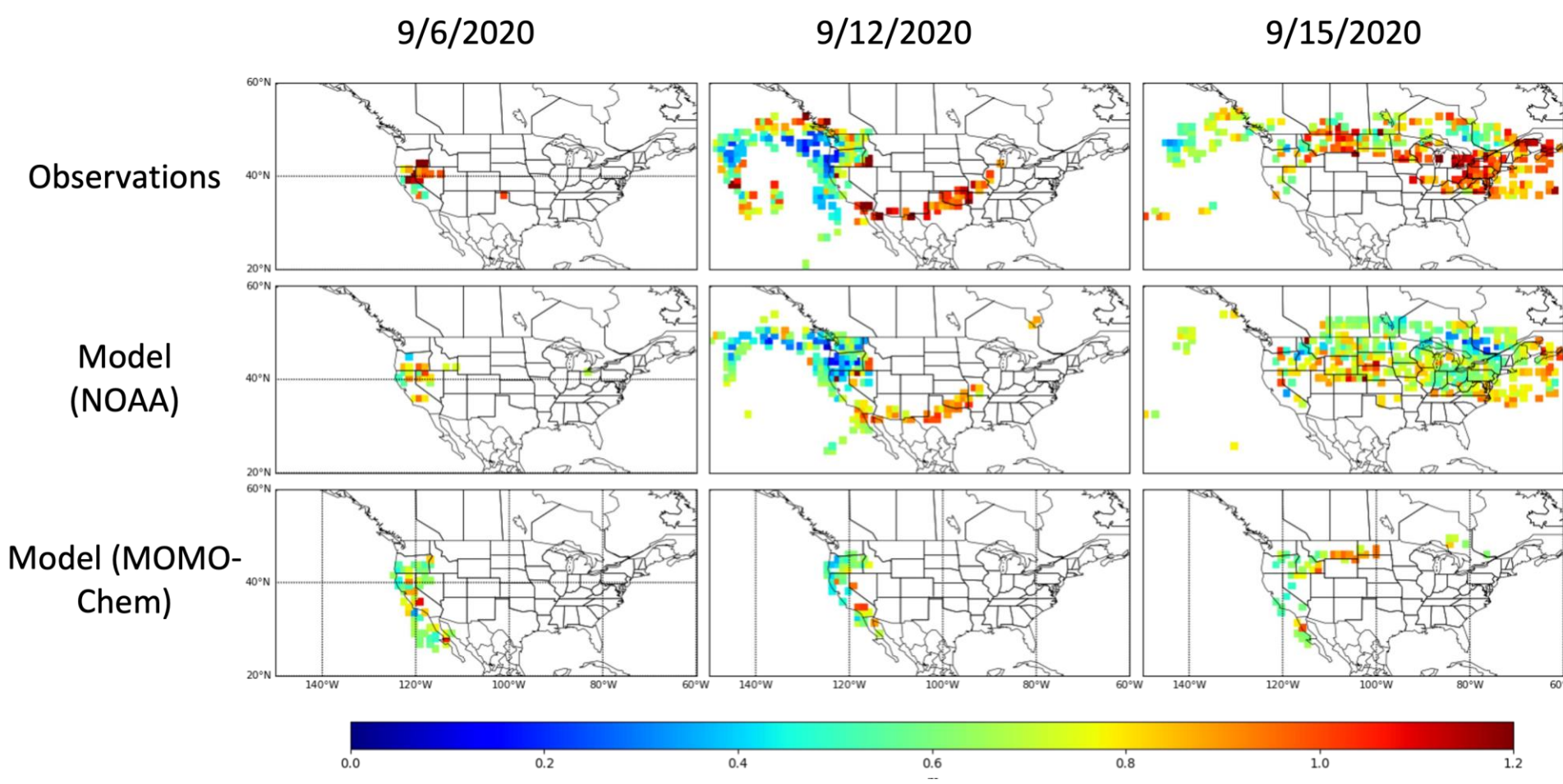
Figure 3: Spatial maps of total CO column ratio between CrIS and TROPOMI (CrIS/TROPOMI) for satellite retrievals (top), NOAA's RAP-Chem simulation (middle), and MOMO-Chem simulation with CrIS and TROPOMI AKs (bottom).
