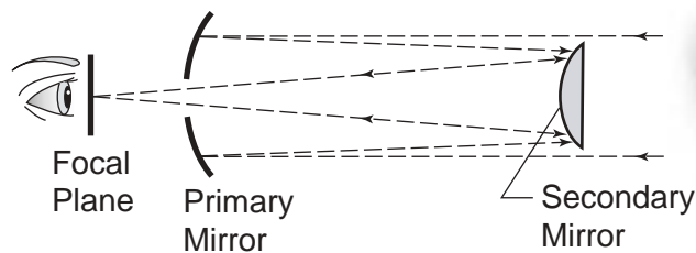
Cassegrain telescope design
