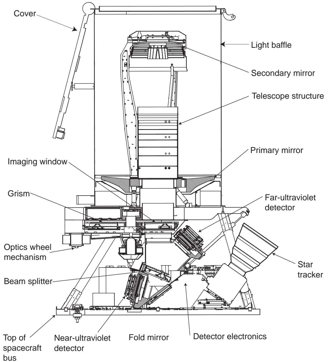
Spacecraft cutaway
