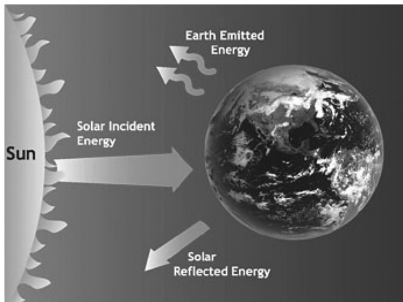
EARTH'S RADIATION BUDGET is a balance between incoming and outgoing radiation.
